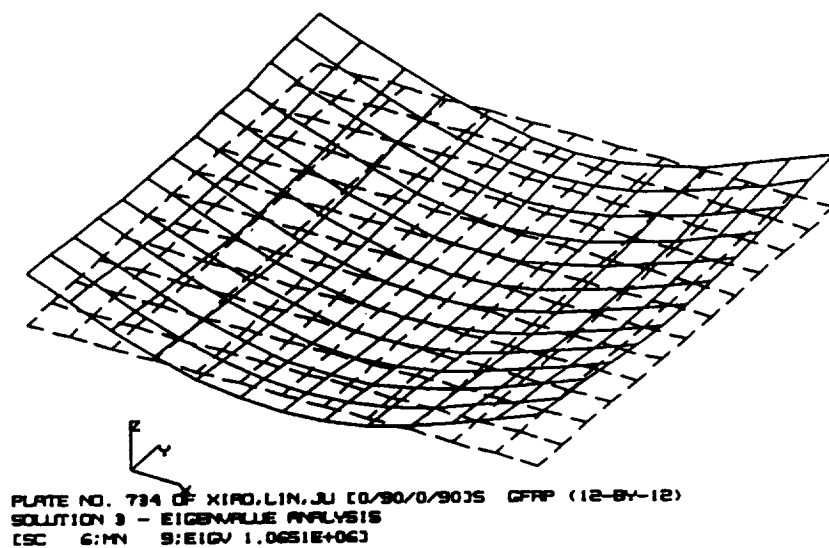
Fig. 3c. Plate 734, Mode 3
