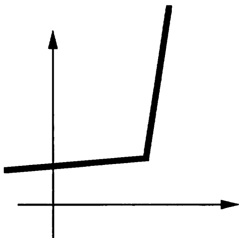
Fig. 6 Force vs. displacement of GAP element
