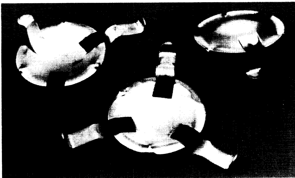
Figure 9: Damaged Valves From the Tray Deck
