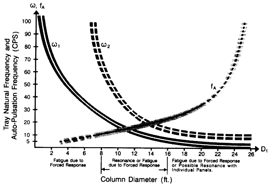
Figure 17: Graphs of the First and Second Tray Natural Frequencies and the Auto-Pulsation Frequency Versus Tray/Column Diameter
