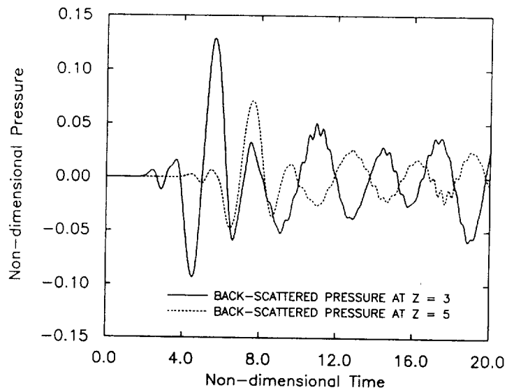
Fig. 6. Time histories of scattered pressure.
