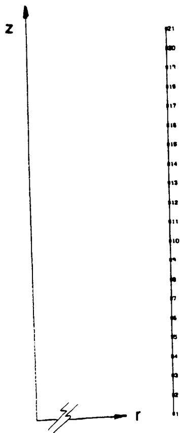
Figure 2b Conical Shell Finite Element Model of Thin-Walled Cylinder
