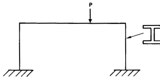
FIGURE 8. PLANE FRAME SUBJECTED TO POINT LOAD (EXAMPLE 4)
