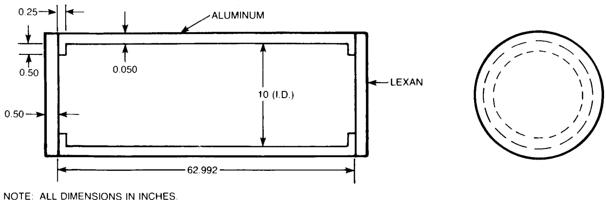
Fig. 1. Cylindrical Shell with Flat End Plates.
