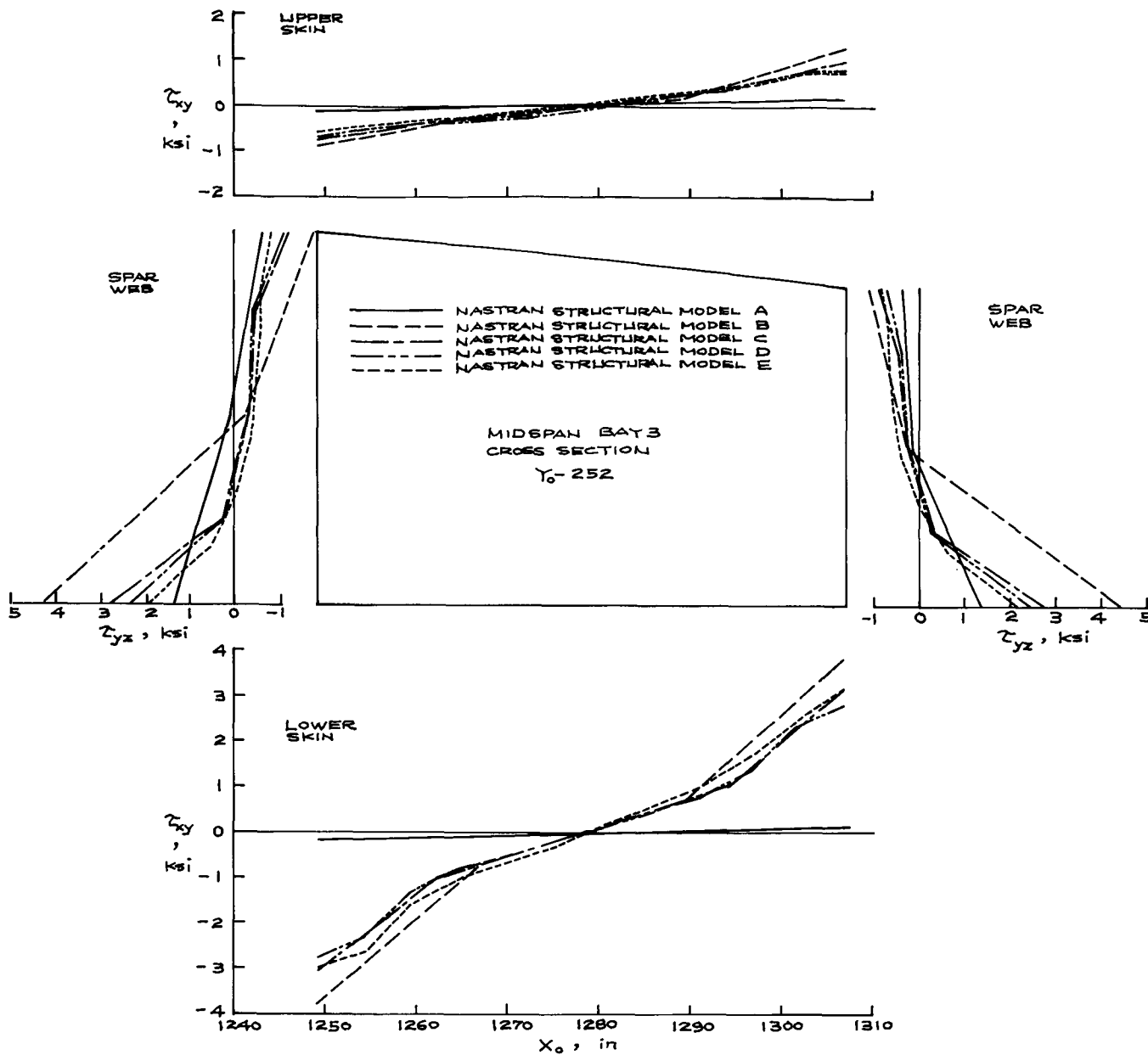
Figure 18. Distributions in the Y 0 -252 plane of shear stresses \tau_{xy} and \tau_{yz} in orbiter wing midspan bay 3 calculated using different NASTRAN structural models; time = 1700 sec, STS-5 flight.
