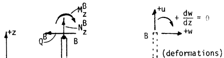
FIGURE 1. FLEXURAL WAVE MODEL FOR SUBMERGED CYLINDRICAL SHELL
