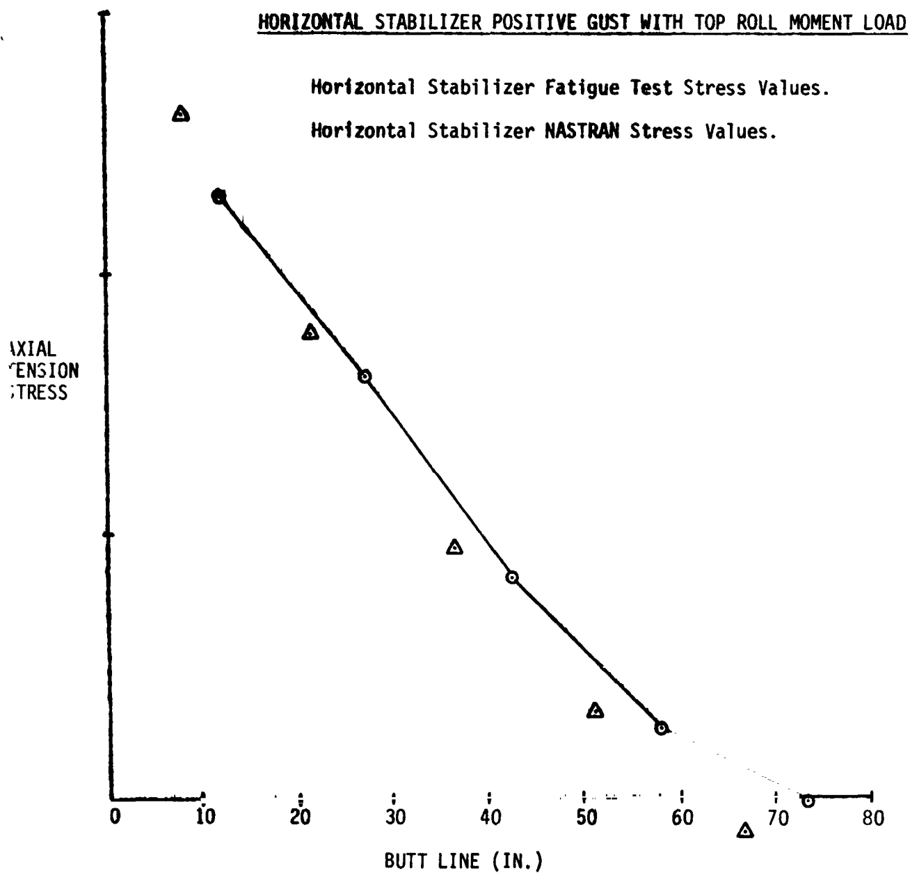
FIGURE 10 - HORIZONTAL STABILIZER REAR SPAR UPPER CAP STRESSES
