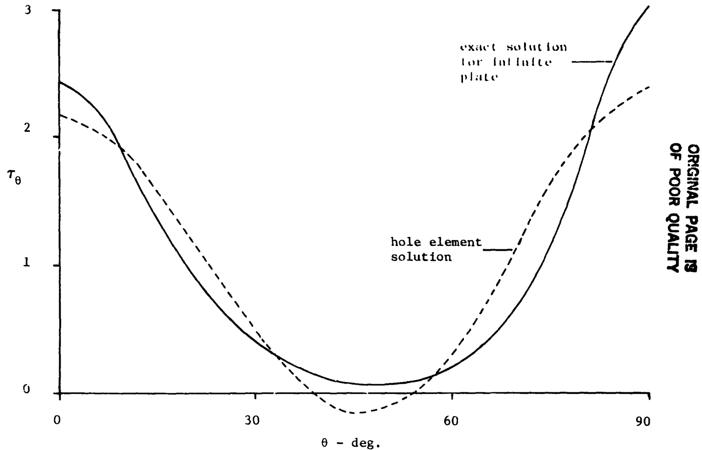
Figure 9. Circumferential Stress at the Hole Boundary for Plywood with Unit Internal Pressure on the Boundary
