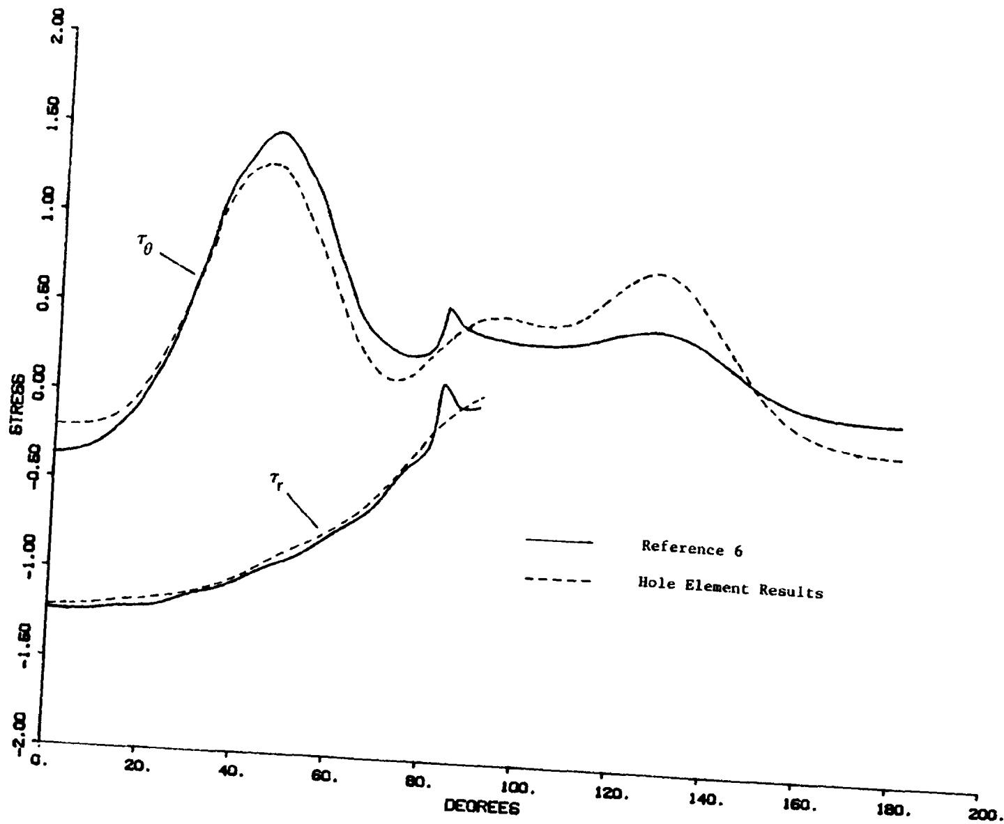
Figure 16. Stresses in the [\pm 45^\circ]_s Laminate
