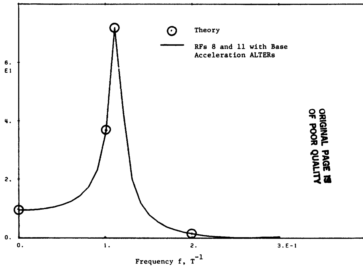
Figure 5. Load Required on Mass m_1 of Example 2 (Figure 3), Frequency Response
