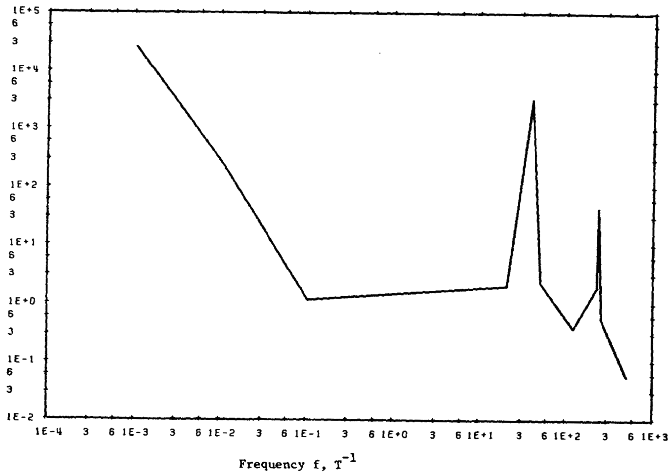
Figure 1. Stress Response \sigma_{xx,1} in Element 2 of Example 1 (Figure 2), RF8 With Large Mass.
