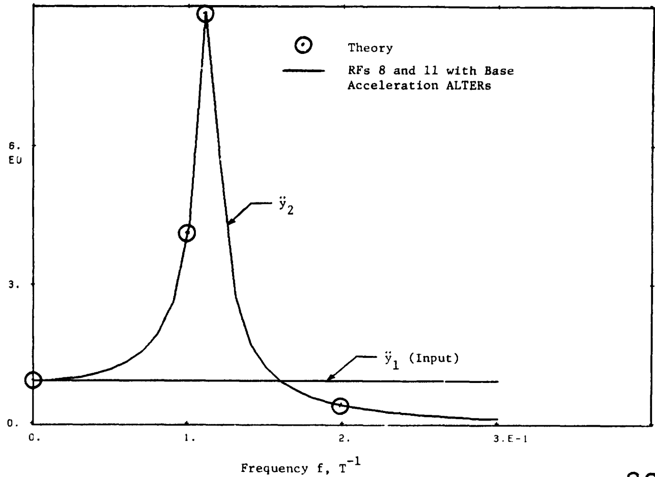
Figure 4. Acceleration Response of Mass m_2 of Example 2 (Figure 3), Frequency Response
