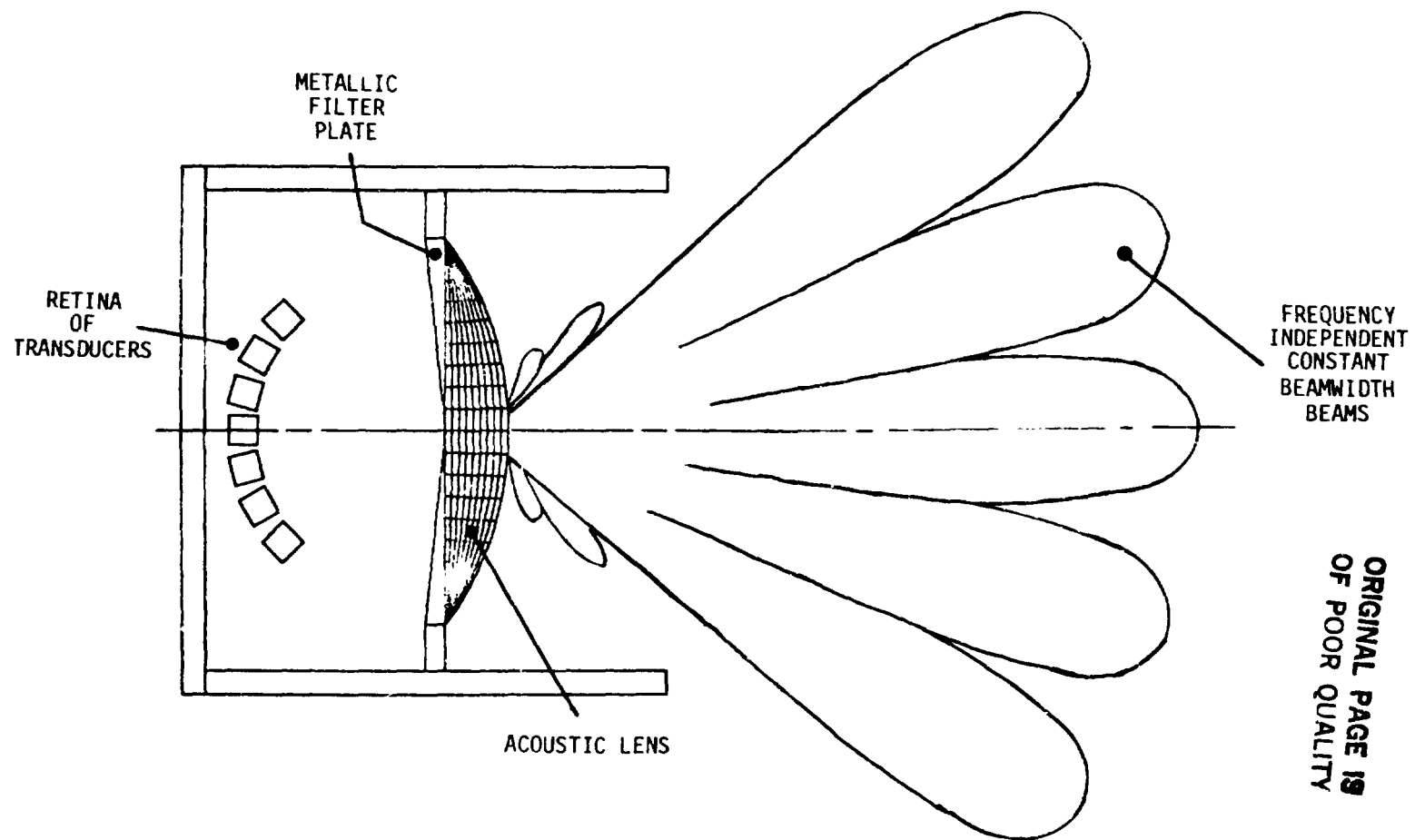
FIGURE 1 A TYPICAL TAPERED FILTER PLATE AND ACOUSTIC LENS CONFIGURATION
