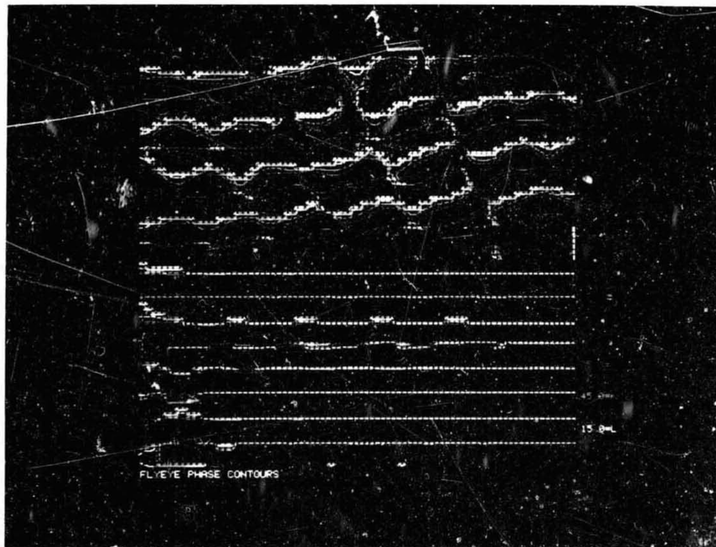
FIGURE 3 COLOR CONTOURS OF THE PHASE DISTRIBUTION THROUGHOUT THE TAPERED FILTER PLATE MODEL
