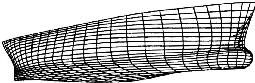
Figure 2 - Ship Hull
